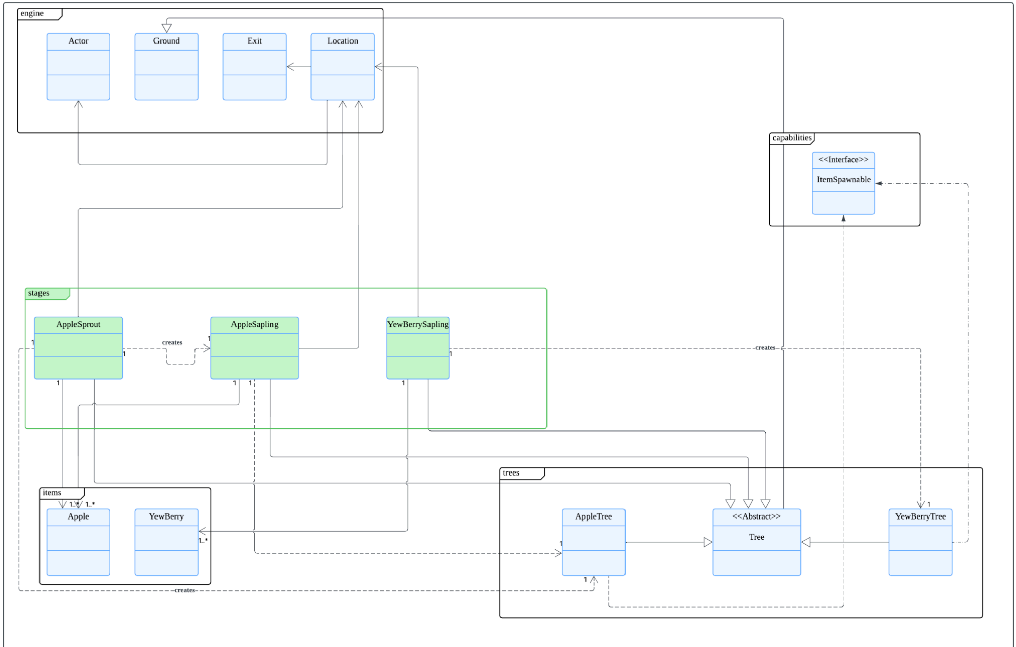
UML Diagram: Tree Growth Stages in Game Environment REQ2
